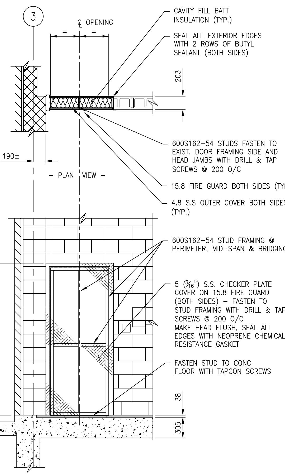
DETAIL - DOOR OPENING CLOSURE SCALE: 1 : 30
