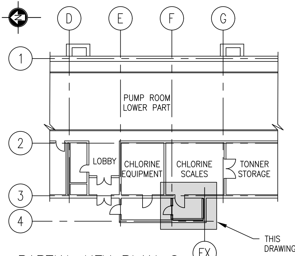
PARTIAL KEY PLAN @ ABOVE ELEVATION 232.528M [762.0'] SCALE: 1 : 250
