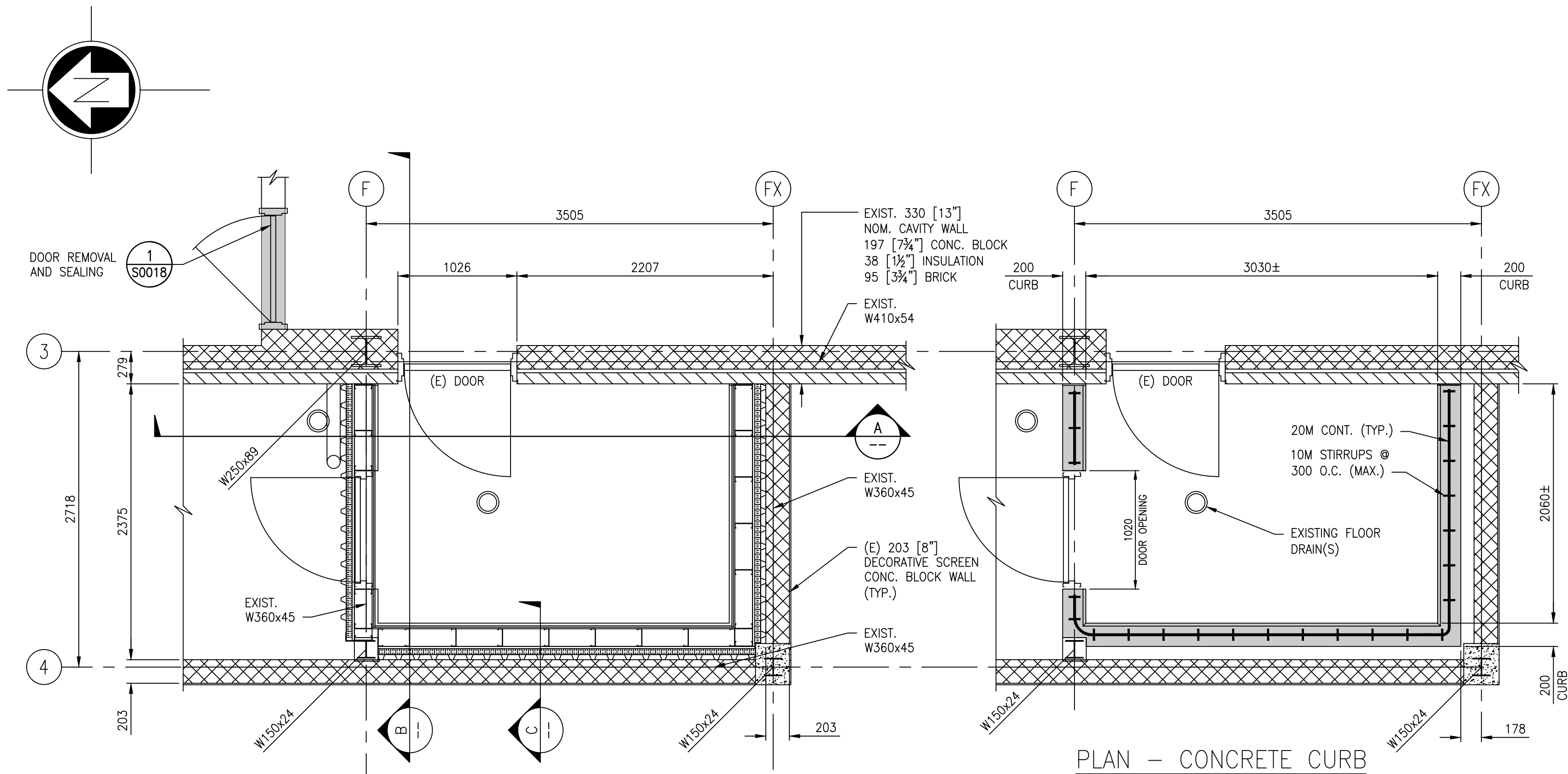
PLAN - SERVICE AREA 314 SCALE: 1 : 30
